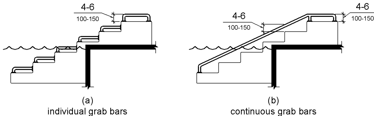
Figure 1009.5.7 Grab Bars
