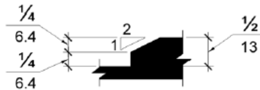
1/2 Inch Change in Level
