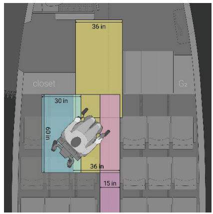
FIGURE 4-11 Space for a wheelchair maneuvering laterally between the aisle and securement area, Boeing 737.
