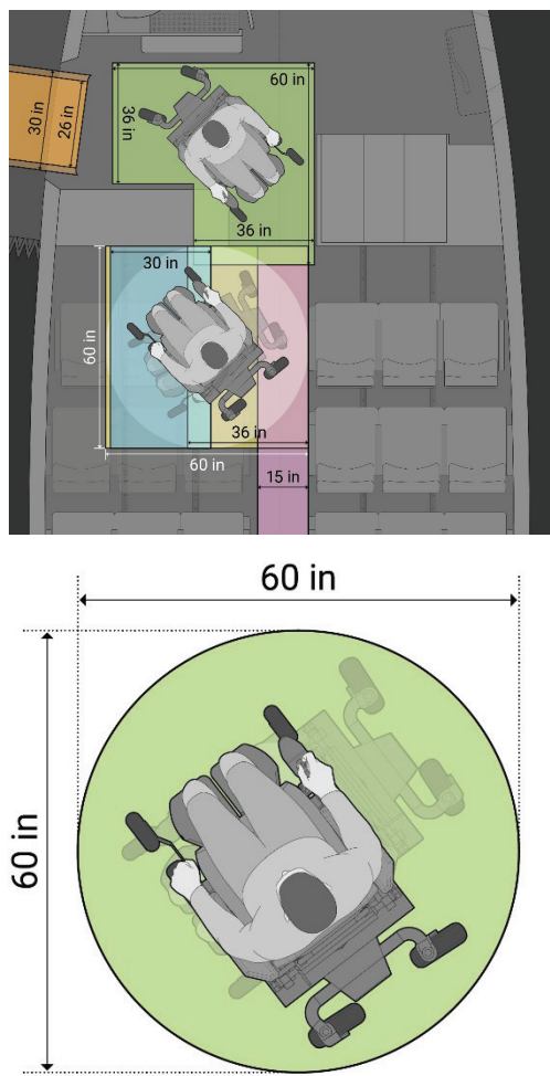
FIGURE 4-7 Minimum space required in the securement area and adjacent aisle to turn the wheelchair around to a front-facing securement position after entering facing forward.
