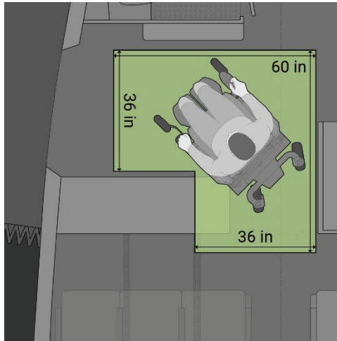
FIGURE 4-4 Space required to turn between the entryway and main aisle.
