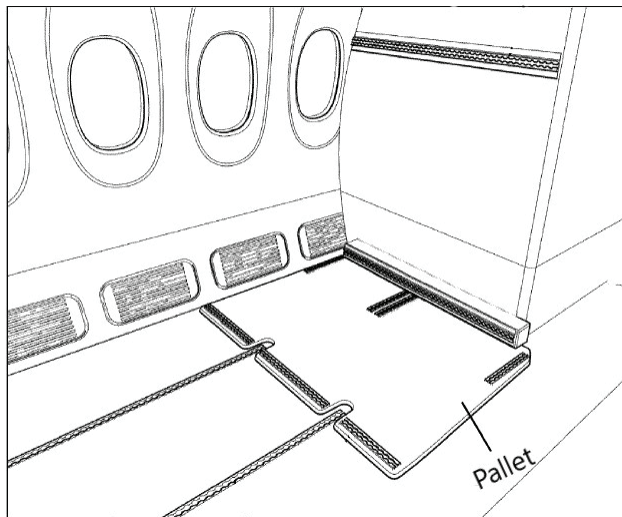
FIGURE 2-9 Aluminum pallet for distributing load across airplane floor structure. SOURCE: European Patent Application. 17
