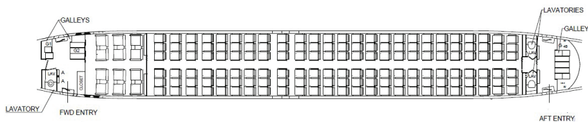
FIGURE 4-8 Boeing 737 interior layout with first class seating.
