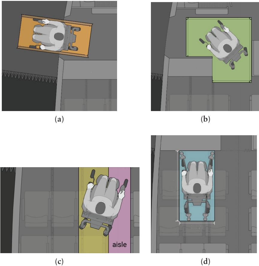
FIGURE 4-1 Wheelchair maneuvers required to access a securement location at the front of the cabin near the forward boarding door: (a) maneuvering through the left forward boarding doorway (gold area indicates the space required for the wheelchair to maneuver); (b) turning between the doorway and main aisle of the passenger compartment (green indicates the space required to perform this maneuver); (c) maneuvering between the main aisle and securement area (yellow indicates the additional space required for this maneuver beyond the aisle); and (d) positioned in a securement location (blue indicates the securement space).
