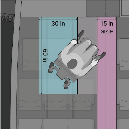
FIGURE 4-5 Space required to maneuver between the aisle and securement location (15-in. aisle width depicted at floor level).
