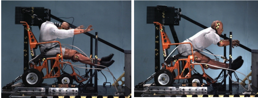
FIGURE 3-3 Peak-of-action photos for a 30-mph, 20-g frontal impact test of WTORS (WC18) using a 185-lb rigid surrogate wheelchair and a mid-size male ATD.
