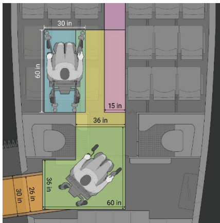
FIGURE 4-13 Space requirements for a wheelchair securement area near the rear door, Boeing 737.
