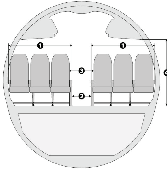
FIGURE 2-8 Cross-section of narrow-body cabin interior with six-abreast seating.
