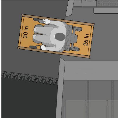
FIGURE 4-3 Minimum clearances required for a wheelchair to maneuver through a cabin boarding door (30-in. clearance partway up the door for clearance of maximum wheelchair width at arm support and 26-in. clearance 1.5 in. above door sill for clearance of wheelbase).
