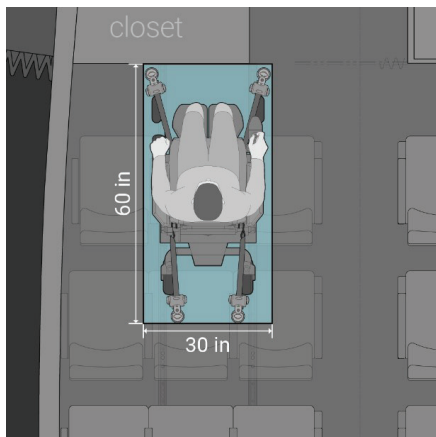
FIGURE 4-12 Space requirements for a wheelchair securement area near the forward loading door, Boeing 737.
