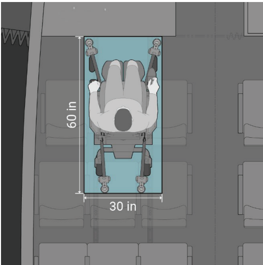
FIGURE 4-6 Space required for the securement area.
