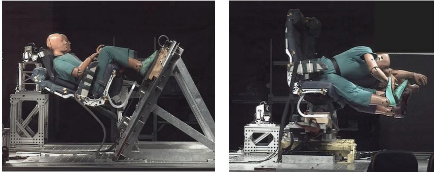
FIGURE 3-1 Dynamic tests (vertical [14 g] and longitudinal [16 g]) to demonstrate compliance with § 25.562.
