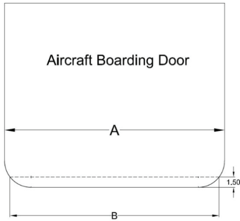
FIGURE 4-2 Boarding doorway width dimensions relevant for determining clearance for a personal wheelchair.
