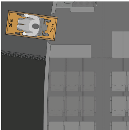
FIGURE 4-9 Forward boarding door clearances, Boeing 737.
