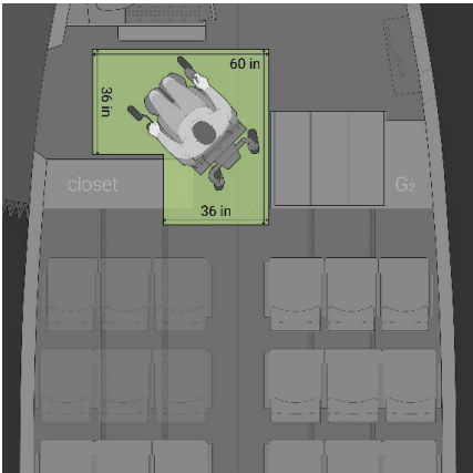
FIGURE 4-10 Turning corridor clearance between the entryway and aisle, Boeing 737.
