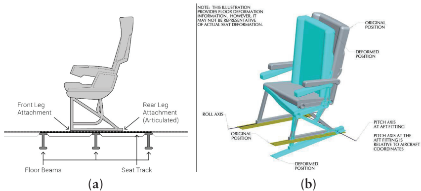
FIGURE 3-2 Illustrations of (a) a typical economy class passenger seat assembly and attachment to seat track, and (b) the floor and seat deformation position.
